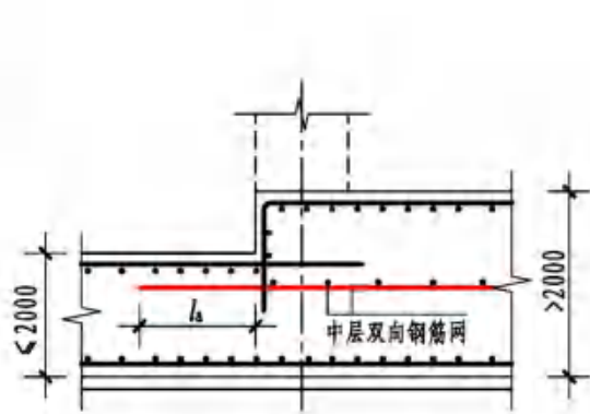
(a) 板顶有高差
